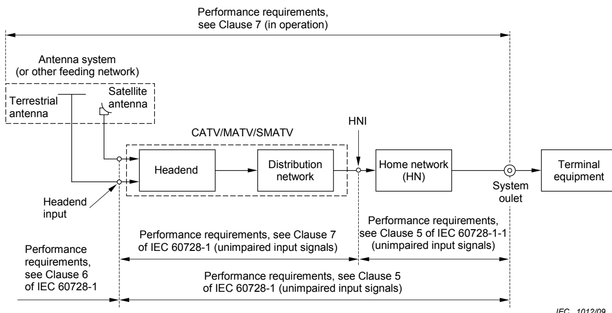
Diagram of the main sections of a CATV/MATV/SMATV cable network and the relevant parts of the IEC 60728-1 series where the requirements are indicated.
